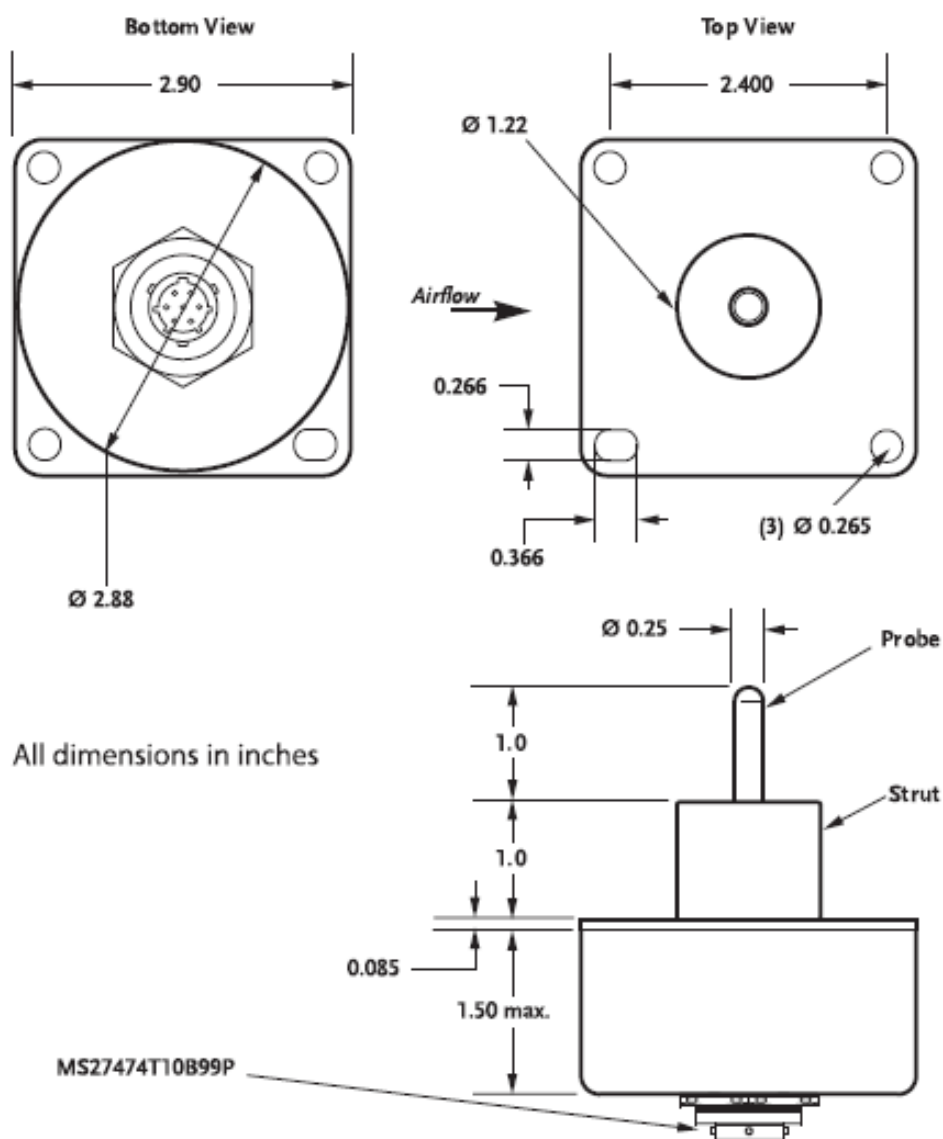
Figure 3 Ice Detector
